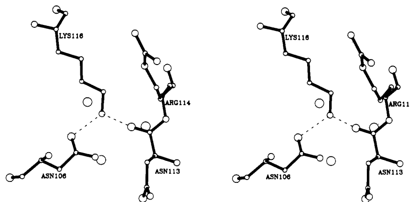
FIGURE 5: Crystalline packing interactions of Lys 116 in the native structure. Shown in stereo is the potential hydrogen-bonding arrangement around N\epsilon' of Lys 116. The open spheres represent the positions of solvent molecules that are within hydrogen-bonding distance of N\epsilon' . Note that N\epsilon' is within 2.9 Å of the carbonyl oxygen of Asn 113, which is located in a symmetry-related molecule in the crystalline lattice. Due to this close contact region between symmetry-related molecules, it is not possible to accommodate a methylated lysine residue in the same conformation. Consequently, the methylated protein crystallized in the space group P2_12_12_1 rather than P4_32_12 leading to a completely different packing arrangement.
